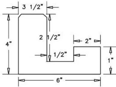
J-CURB (SIDE VIEW)
