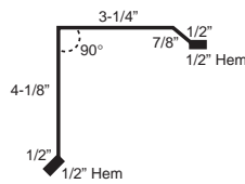
13b 5-1/2" FASCIA TRIM cccBFAH
