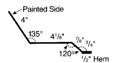
16a END WALL cccB105AH
