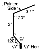
19a TRANSITION FLASHING cccTRANSH
