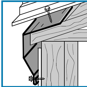
14. Eave Trim – Conceals rafter end for a building with a small eave over-hang.
