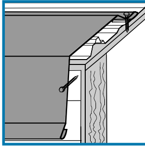
3. Rake Trim – Seals off where end wall panels meet roof panels.
