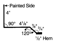
11 SIDE WALL TRIM ccc105AH
