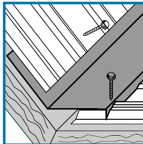
19b. Notched Transition Flashing – Prevents leaks when you have change in roof pitch.
