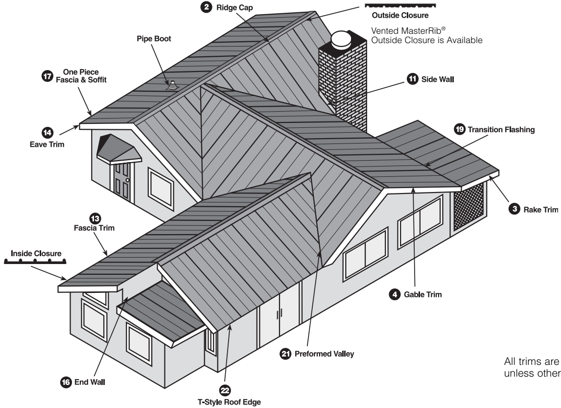
3 RAKE TRIM cccRAKEH
