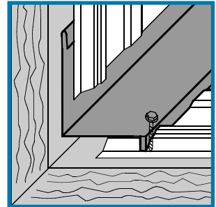
16b. Notched End Wall – Prevents leaks where an end wall connects to a lower roof.
