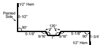
20b NOTCHED GAMBREL FLASHING (41") cccNGAMBREL29
