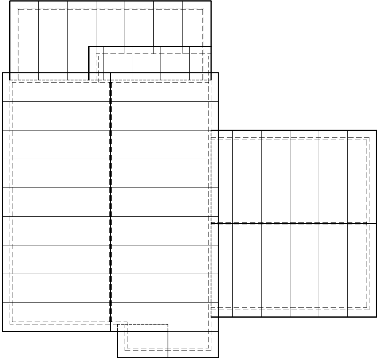
Roof Panel Plan \frac{3}{16}'' = 1'-0''
