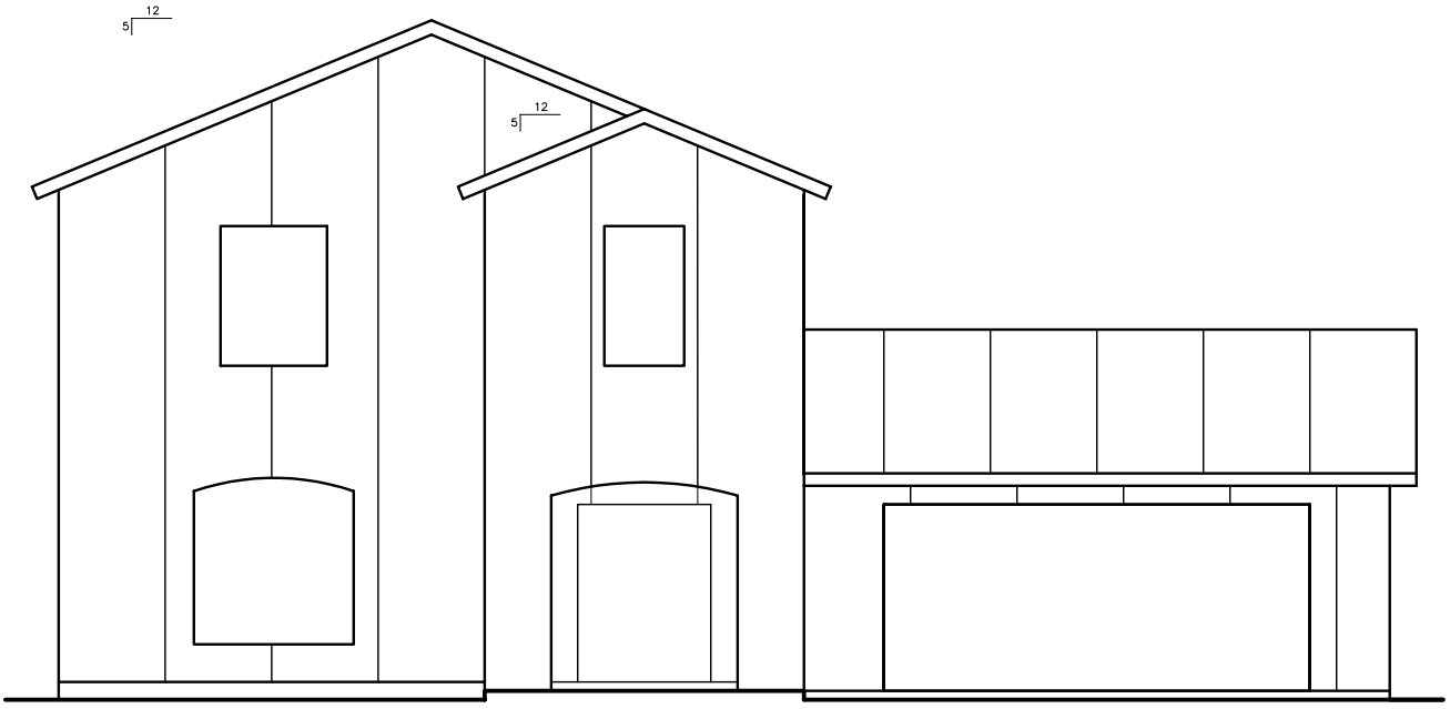
Front Elevation 3/16'' = 1'-0''
