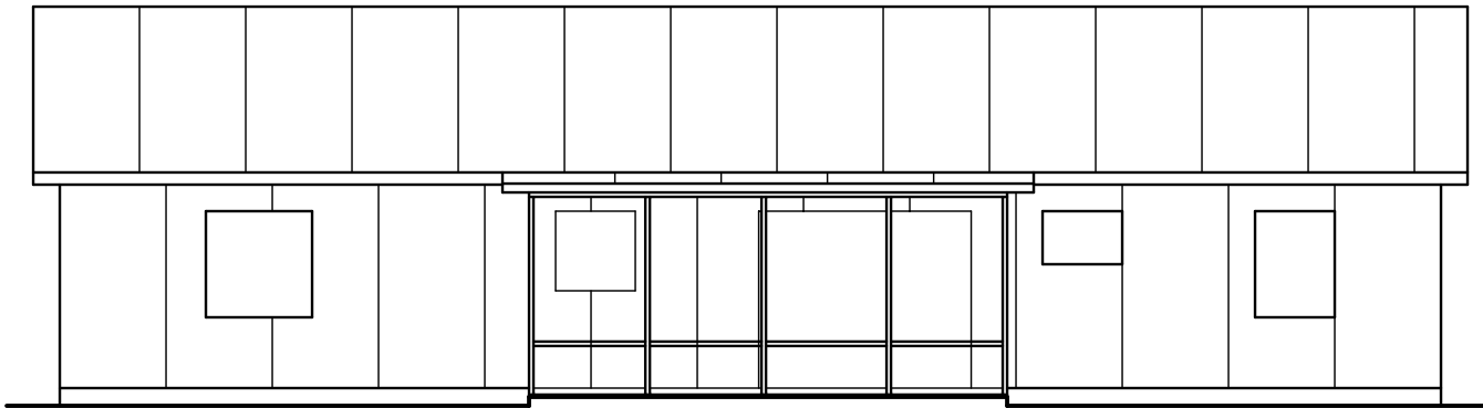
Back Elevation 1/8'' = 1'-0''
